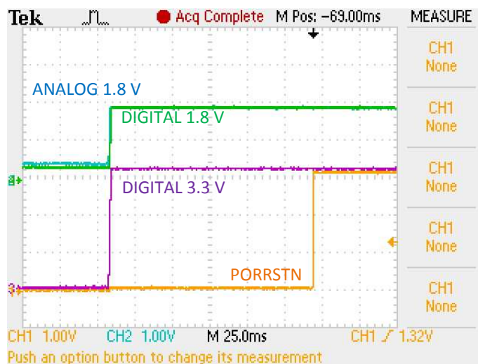
Figure 3-3. PORRST Signal Power-Up Sequence Example
